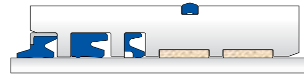
Configuration K11-K22+ Back-Up Ring-K35-K75-K84
